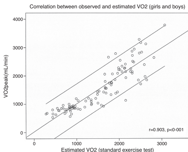
Figure 3 The association between the linear regression model (estimated VO 2 ) and actual VO 2 values. This model was calculated using body surface area (BSA), exercise time (ET), gender and heart rate reserve (RHR).
